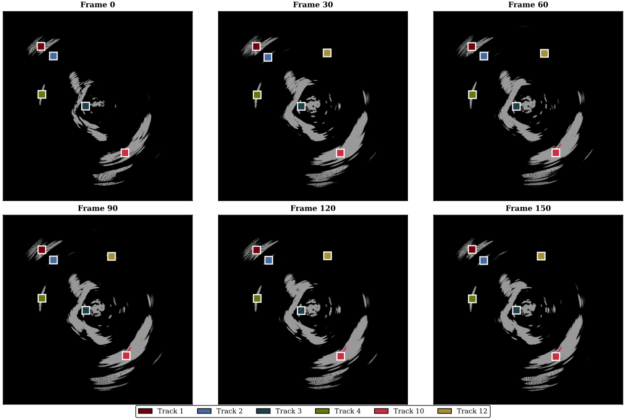
Fig. 8 Tracking sequence showing vessel positions across consecutive radar sweeps. Track identifiers remain consistent despite intermittent detections, demonstrating the effectiveness of the gap recovery mechanism.
