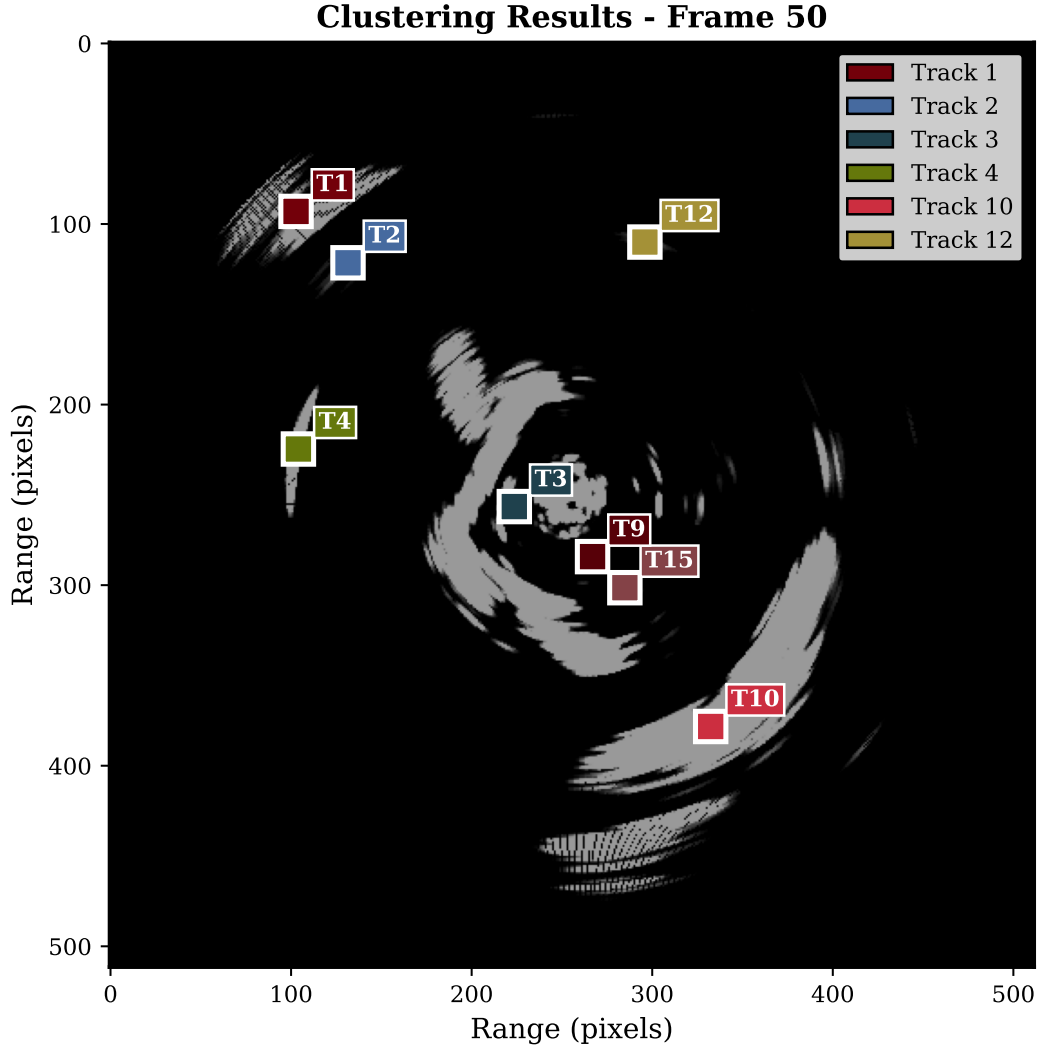
Fig. 4 ST-DBSCAN clustering result on a multi-vessel scene. Each cluster is assigned a unique color; noise points are shown in gray. The algorithm successfully separates individual vessel returns from sea clutter.
