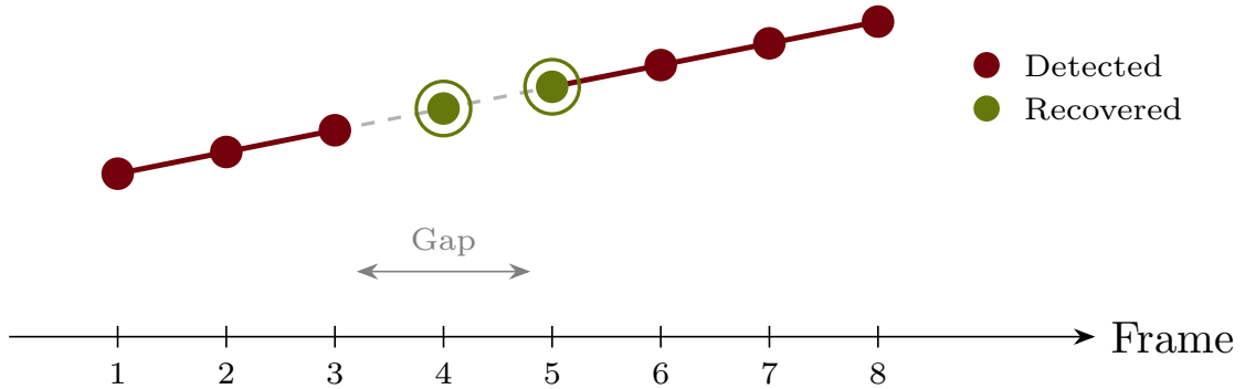
Fig. 5 Gap recovery mechanism. When a vessel temporarily disappears (frames t_1 to t_2 ), the algorithm reconnects clusters based on centroid proximity, maintaining track identity across brief dropouts.
