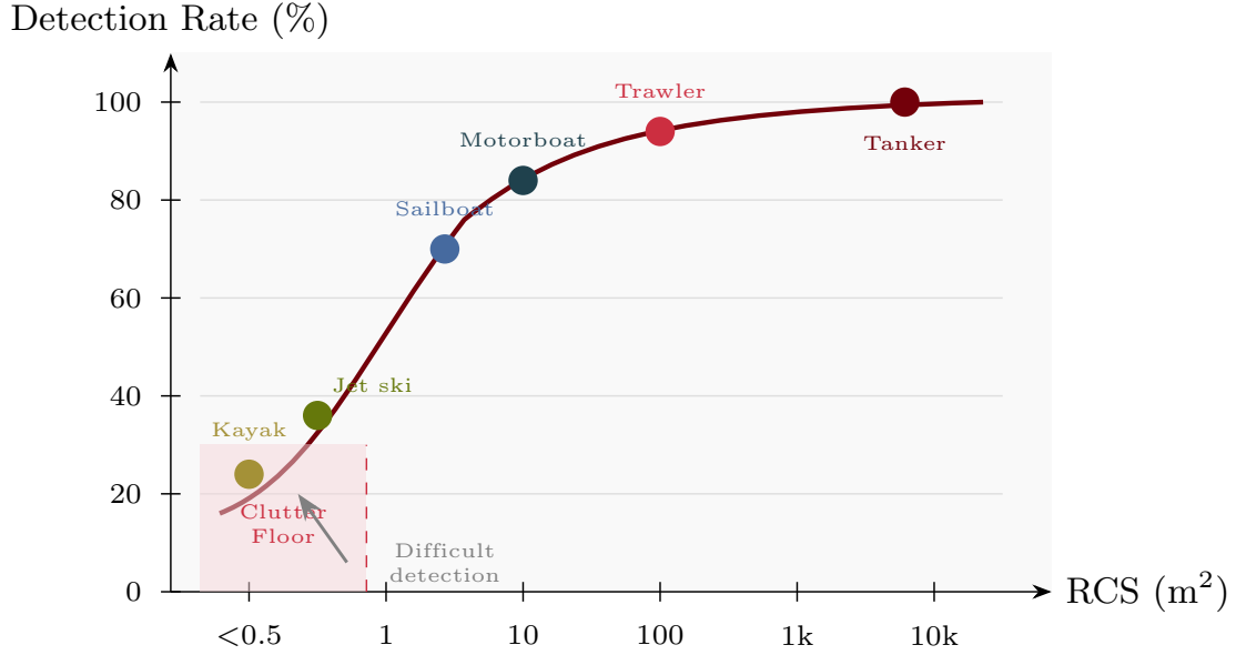
Fig. 14 Radar cross-section (RCS) variability analysis. Target returns fluctuate significantly due to aspect angle changes and sea state variations, motivating the need for adaptive clustering parameters.
