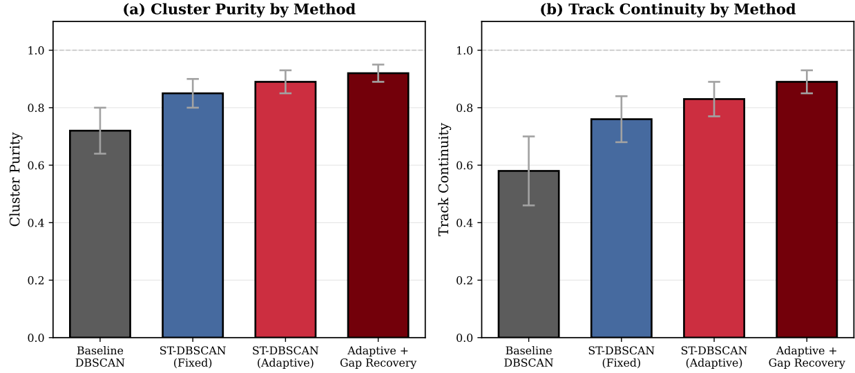
Fig. 19 Ablation study comparing cluster purity and track continuity across system configurations. Each component contributes incrementally to overall performance.
