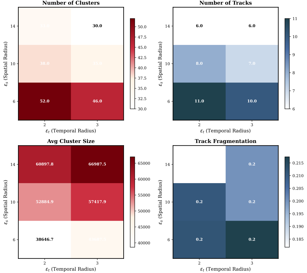
Fig. 18 Parameter interaction heatmaps showing the combined effect of spatial radius \epsilon_s and temporal radius \epsilon_t on clustering and tracking metrics.
