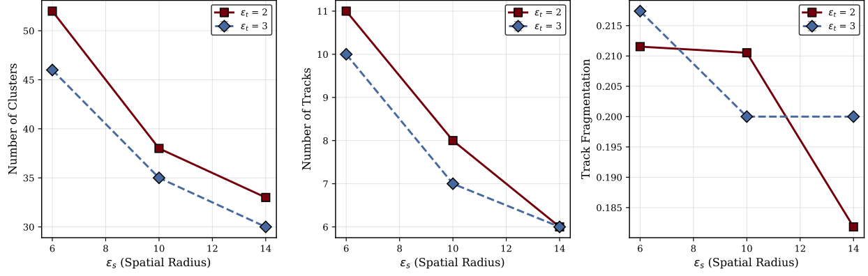
Fig. 16 Sensitivity of tracking metrics to spatial radius \epsilon_s for different temporal radii \epsilon_t . Larger spatial radii produce fewer, larger clusters with reduced fragmentation.
