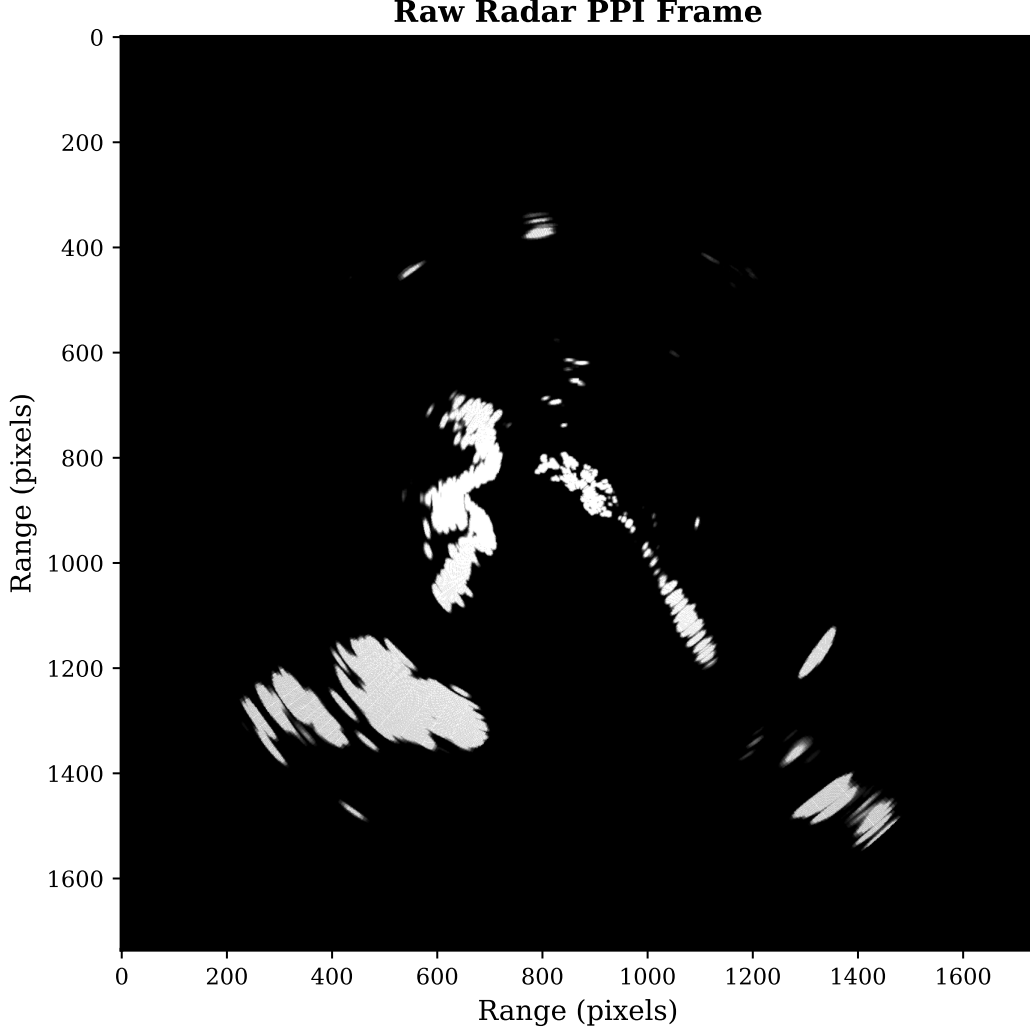
Fig. 3 Raw radar return example from the Furuno DRS-NXT unit. Multiple vessel returns are visible against varying sea clutter intensity, demonstrating the challenging detection environment.
